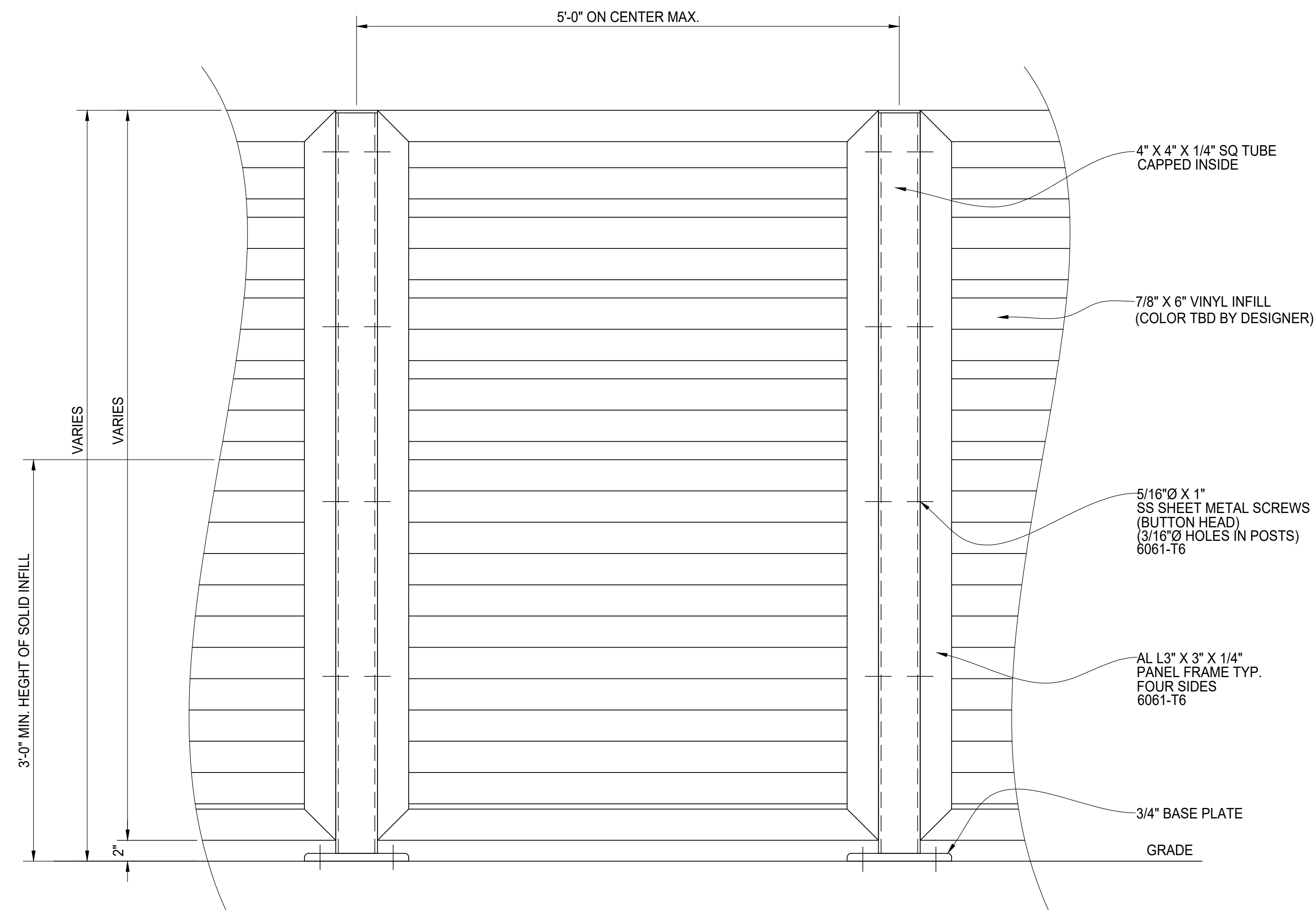
ELEVATION VIEW
