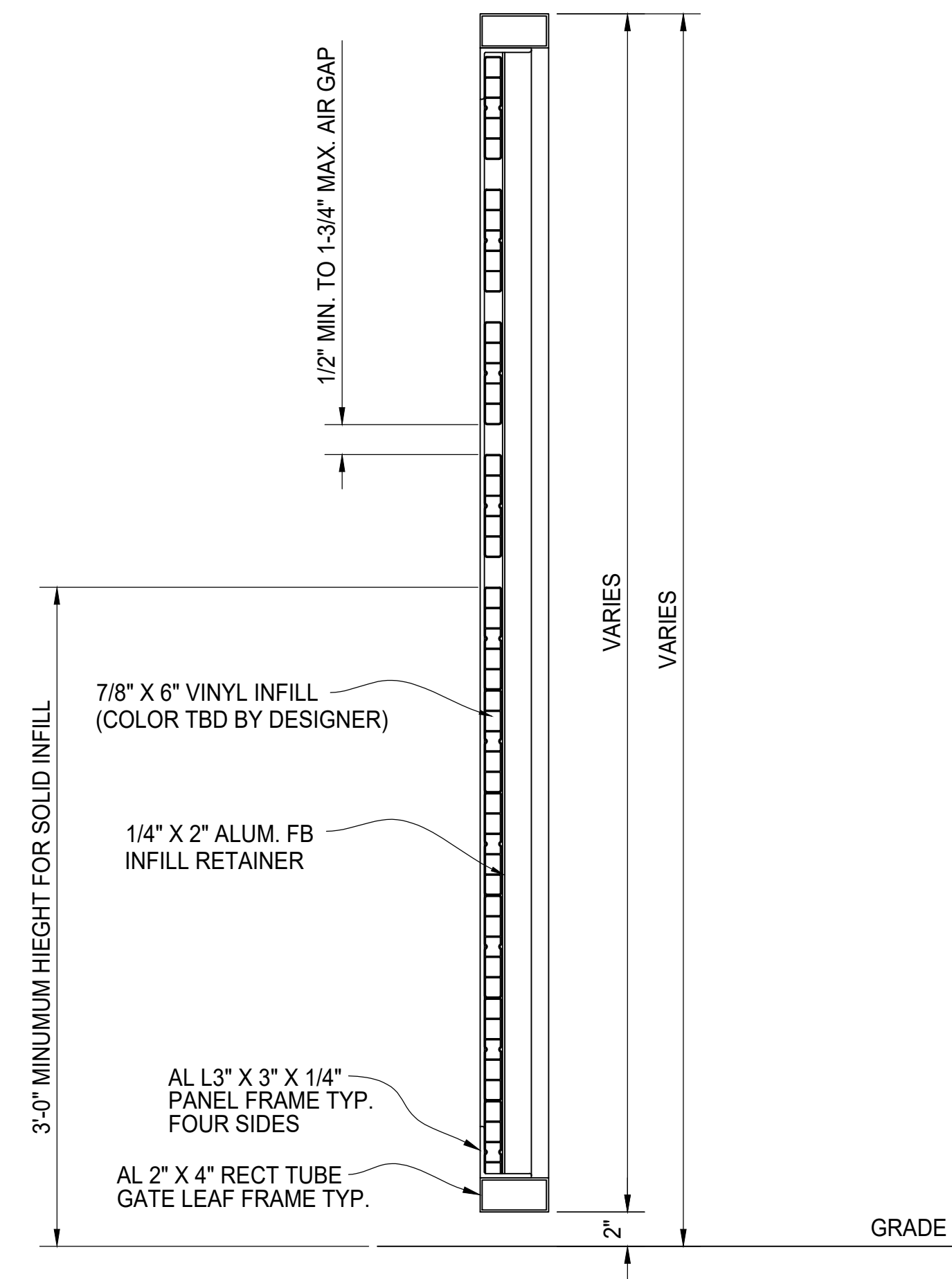
TYPICAL GATE SECTION
