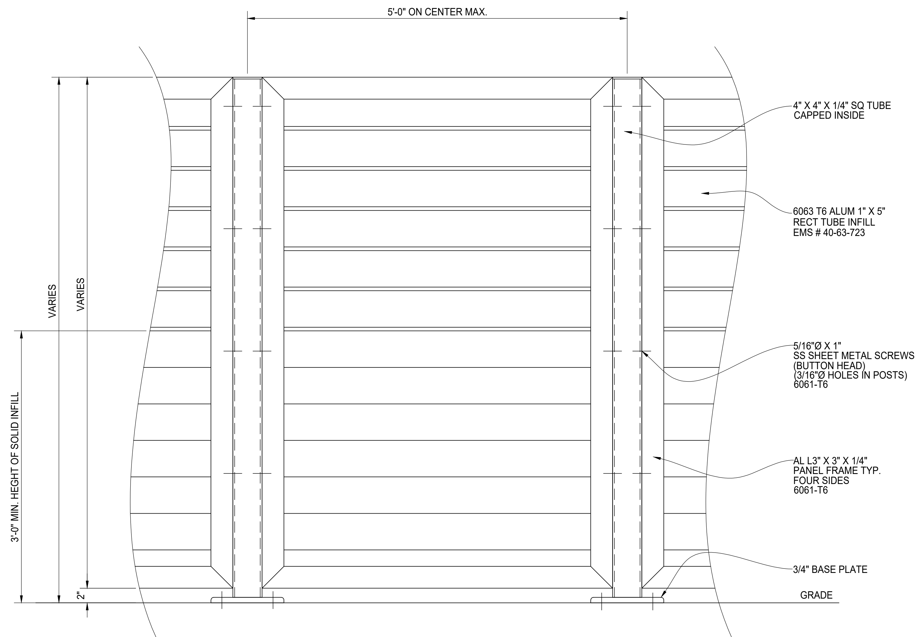
ELEVATION VIEW TYPICAL PANEL DETAIL
