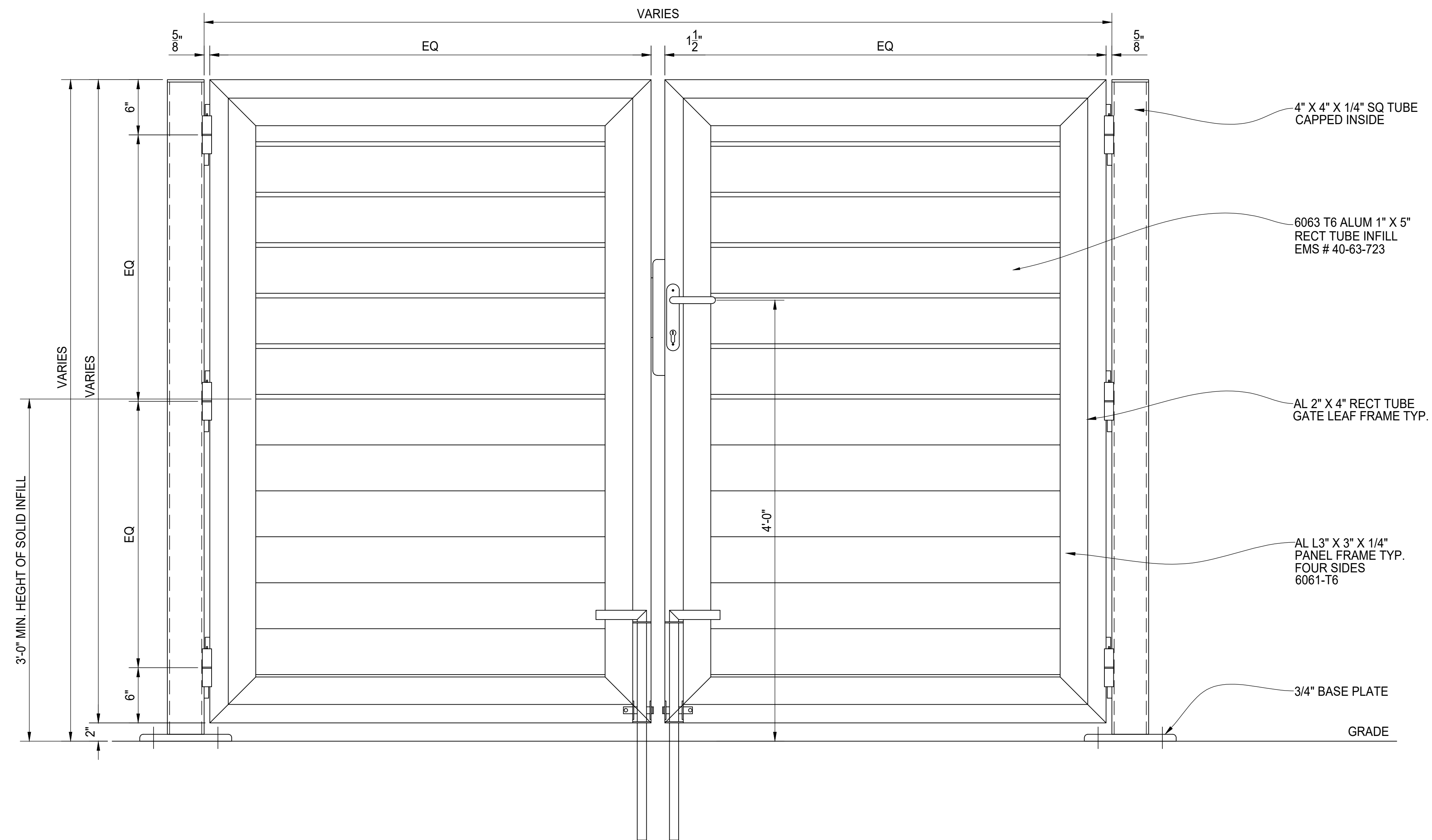
ELEVATION VIEW
